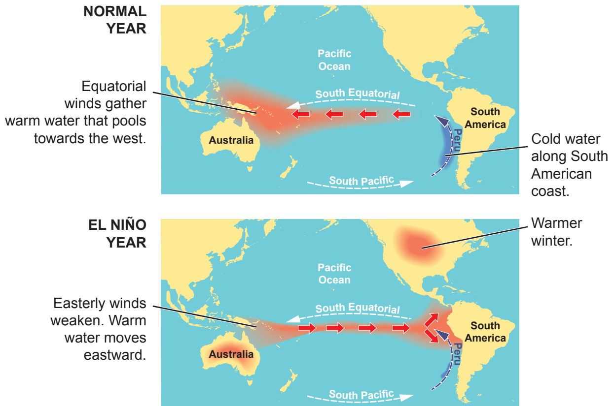
Fig. 1 Maps showing atmospheric and ocean circulation in the Pacific during a normal year and an El Niño year.
